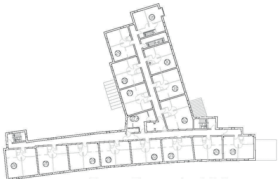
First Floor 1:500
